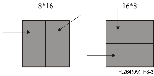
Figure 8-3 – Directional segmentation prediction (informative)
